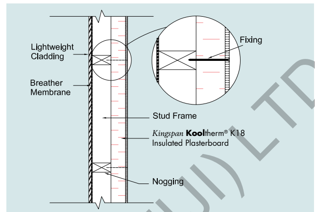
Figure 7 Side elevation - Lightweight cladded stud wall with Kingspan Kooltherm ® K18 Insulated Plasterboard
