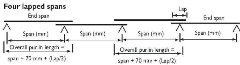
Four lapped span: Z/C 15019 (kN/m)
