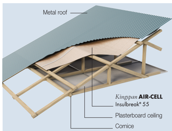
Figure 8 Kingspan AIR-CELL Insulbreak® 55 in a metal roof with an attic space and flat ceiling
